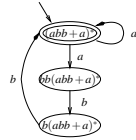
Figure 3: A NFA for (abb+a)^* .
